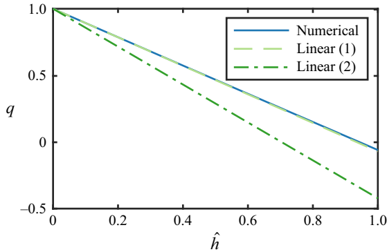
Figure 6. Dependence of growth rate factor q on the thickness \hat{h} for \hat{S} = 0.3 . The solid blue curve corresponds to the full numerical solution. The dashed light green line shows a first linear approximation given by (4.1). This agrees very well with the full numerical solution. The dot-dashed darker green line shows a second alternative linear approximation q = q_0 - \hat{h}/(1 - \hat{S} + \theta_e) which does not agree with the numerical calculation.
