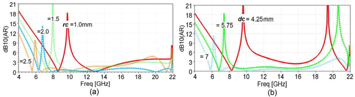
Figure 3. AR graphs (normal incident) of the proposed LP-CP converter (without FSS2) for different values of (a) r_c (when d_c=7 mm and h_1=1.55 mm) and (b) d_c (when r_c=2.5 mm and h_1=1.55 mm) in FSS1. AR = axial ratio; CP = circularly polarized; FSS = frequency-selective structures; LP = linearly polarized.
