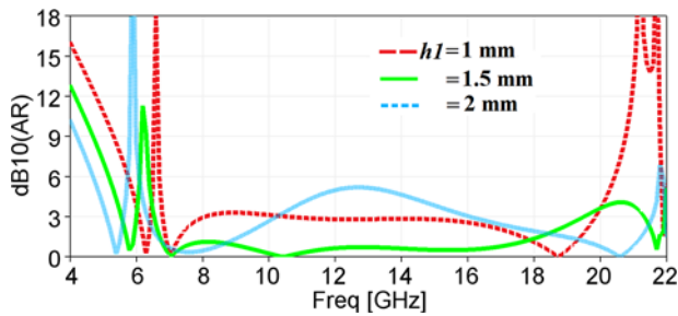
Figure 4. AR graphs (normal incident) of the proposed LP-CP converter (without FSS2) for different values of h_1 in FSS1 (when d_c=7 mm and r_c=2.5 mm). AR = axial ratio; CP = circularly polarized; FSS = frequency-selective structures; LP = linearly polarized.
