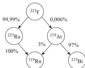
Figure 2 Cascade of radioactive decomposition of ^{223}\text{Fr} .
