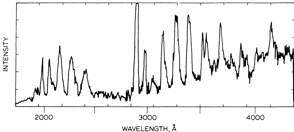
Fig. 1. Ultraviolet spectrum of Mars upper atmosphere. A nominal wavelength scale is shown on the abscissa. The ordinate is an arbitrary intensity scale uncorrected for the spectral response of the instrument. A number of spurious noise pulses have been edited out of this spectrogram.
