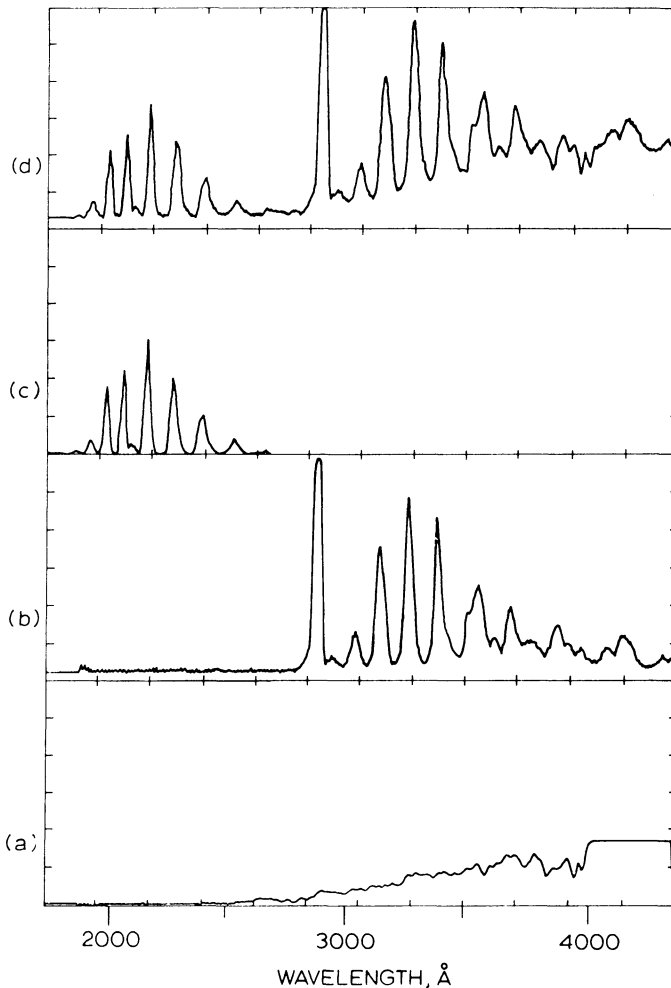
Fig. 2. Synthesis of comparison spectrum. (a) Off-axis light component from Mars disc. (b) Carbon dioxide spectrum from laboratory electron impact experiment. (c) Carbon monoxide spectrum from theoretical calculation of fluorescence scattering. (d) Composite spectrum synthesized by adding a, b, and c.
