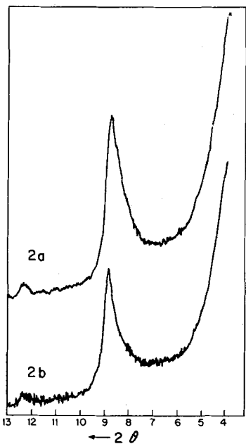
Fig. 2. Diffractometer trace of sample TW1675, (a) air-dried, (b) glycolated.
