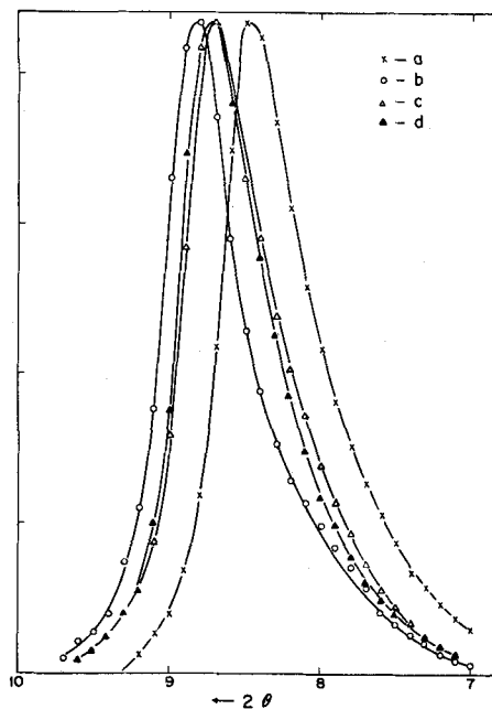
Figs. 4a-d. Derived from curves 3a-d by dividing by the appropriate values of F^2LP (single crystal).
