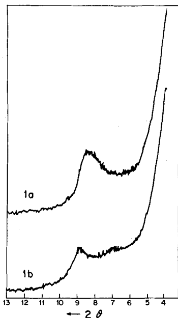
Fig. 1. Diffractometer trace of sample TW834, (a) air-dried, (b) glycolated.
