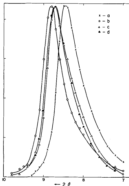
Fig. 3. Intensities obtained by point-by-point counting, subtraction of background and normalizing of sample TW1675, (a) in an air-dried state, (b) glycolated, (c) heated at 110°C, and (d) heated at 200°C.
