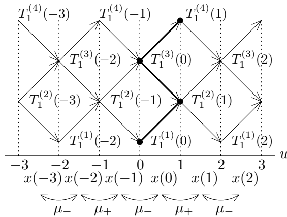
Figure 2: Relation of x(u) and T_1^{(a)}(u) for X_r = A_4 . The thick quiver corresponds to the initial seed (Q, x(0)) of the cluster algebra \mathcal{A}_Q , where we take I_+ = \{1, 3\} , I_- = \{2, 4\} .
