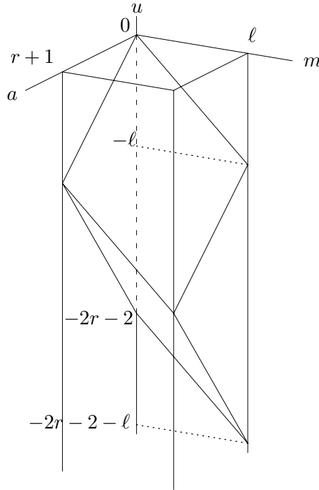
Figure 4: The prism P defined in (5.17)
