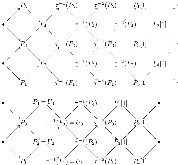
Figure 3: The Auslander-Reiten quivers of \mathcal{D}_Q for X_r = A_5 (the above) and A_4 (the below)
