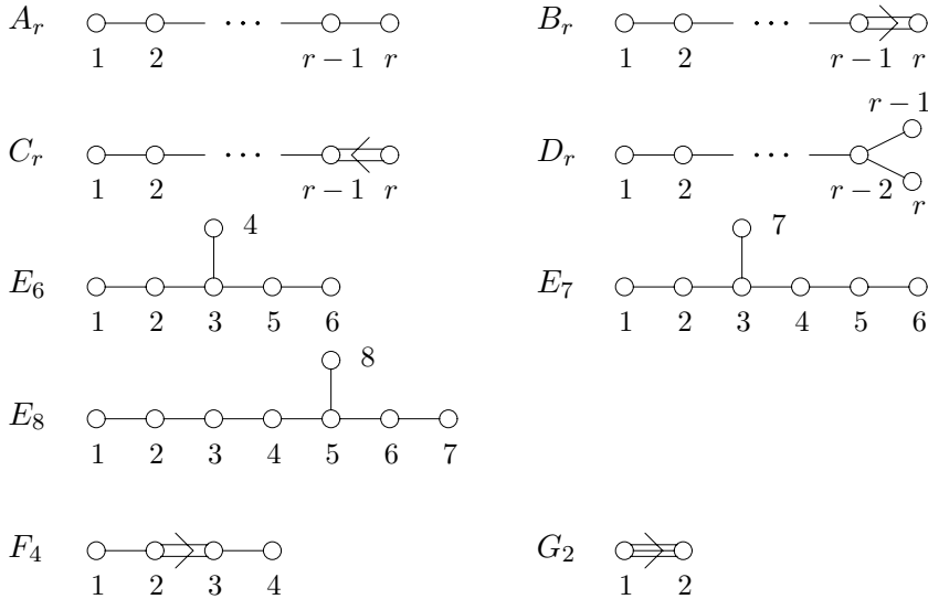
Figure 1: The Dynkin diagrams X_r and their enumerations
