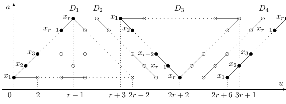
Figure 5: The fundamental domain of \tau^{(a)}(u; X) for \mathcal{T}_2(A_r) . The solid circles in D_1 are identified with the initial variables of \mathcal{T}_2(A_r)_+ .
