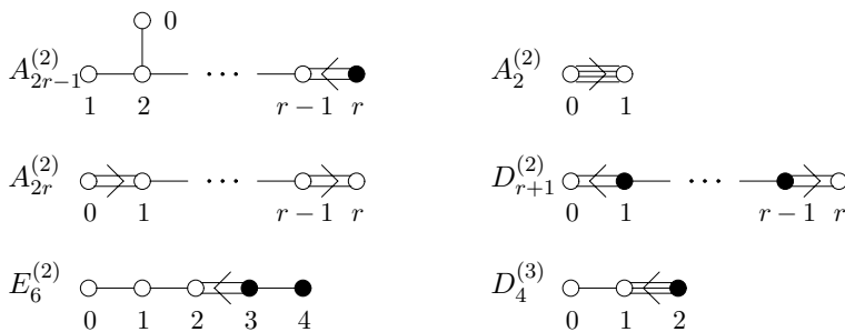
Figure 8: The Dynkin diagrams X_N^{(\kappa)} of twisted affine type and their enumerations by I_\sigma \cup \{0\} . For a solid node a , \sigma(a) = a (i.e., \kappa_a = \kappa ) holds.
