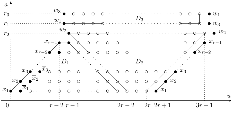
Figure 7: The half of the fundamental domain of \tau_m^{(a)}(u; X) for \mathcal{T}_2(B_r)
