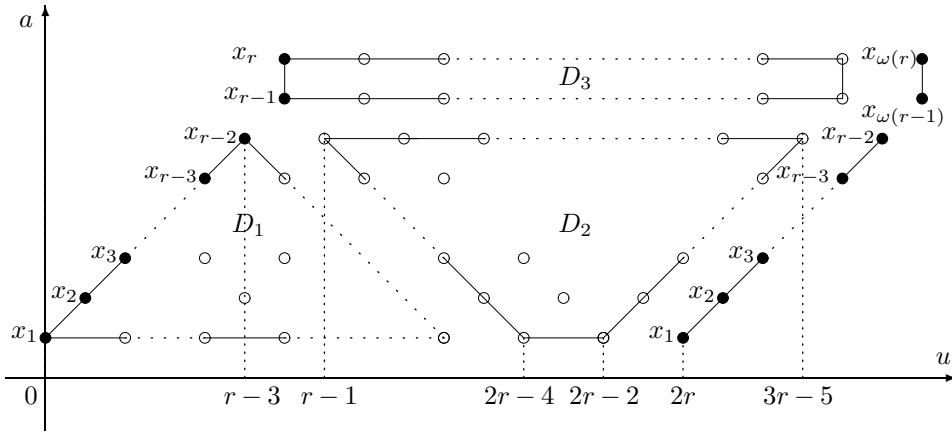
Figure 6: The half of the fundamental domain of \tau^{(a)}(u; X) for \mathcal{J}_2(D_r)
