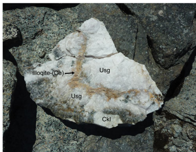
Fig. 2. Example of the paragenesis of illoqite-(Ce) with the brown 'band' running through the rock being weathered illoqite-(Ce). Ussingite (Usg) and chkalovite (Ckl) are marked respectively.
