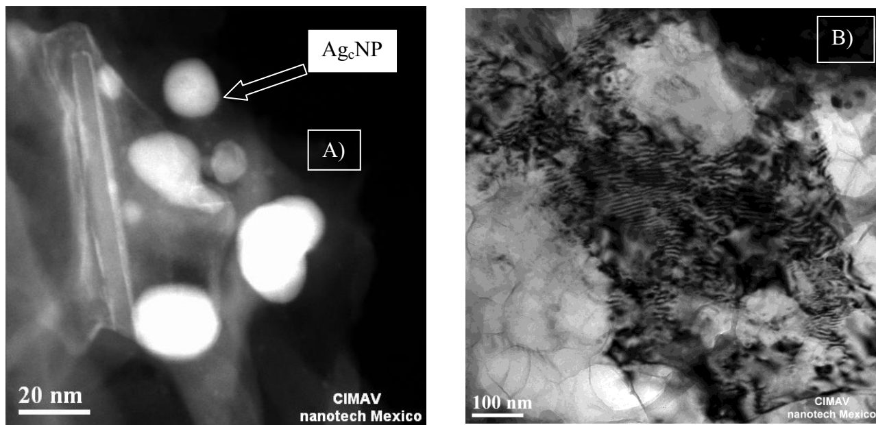
FIG. 1. Precipitates morphology co existing with Ag c NP and dislocation interacting with Ag c NP, aged at 463K
