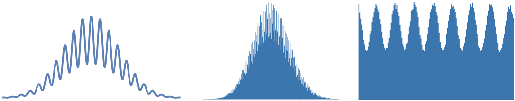
Figure 1. On the left is a cartoon of (one possibility for) the probability mass function of e(G[U]) for a Ramsey graph G and a uniformly random vertex subset U : The large-scale behavior is Gaussian, but on a small scale we see many smaller Gaussian-like curves. The two images on the right are two different histograms at different scales, obtained from real data (namely, from two million independent samples of a uniformly random vertex subset in a graph G obtained as an outcome of the Erdős–Rényi random graph \mathbb{G}(1000, 0.8) ).
