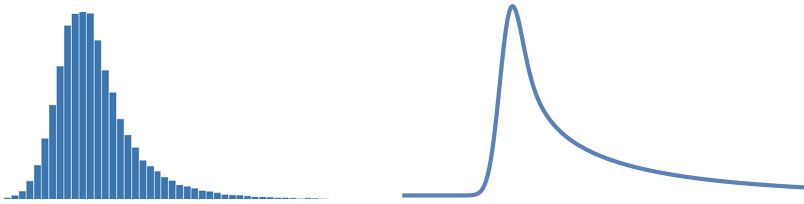
Figure 2. On the left, we obtain G as a disjoint union of two independent Erdős–Rényi random graphs \mathbb{G}(800, 0.96) , and we consider 500,000 independent samples of a uniformly random vertex subsets U with exactly 800 vertices. The resulting histogram for e(G[U]) may look approximately Gaussian, but closer inspection reveals asymmetry in the tails. This is not just an artifact of small numbers: The limiting distribution comes from a nontrivial quadratic polynomial of Gaussian random variables. Actually, it is possible for the skew to be much more exaggerated (the curve on the right shows one possibility for the limiting probability mass function of e(G[U]) ), but this is difficult to observe computationally, as this shape only really becomes visible for enormous graphs G .
