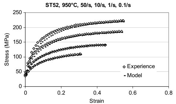
Fig. 3. Effect of strain rate is also well reproduced (uniaxial compression data, 0.2% C, 1.5% Mn, 0.2% Si grade deformed at 950 °C for strain rates varying from 0.1 to 50 s -1 ).
