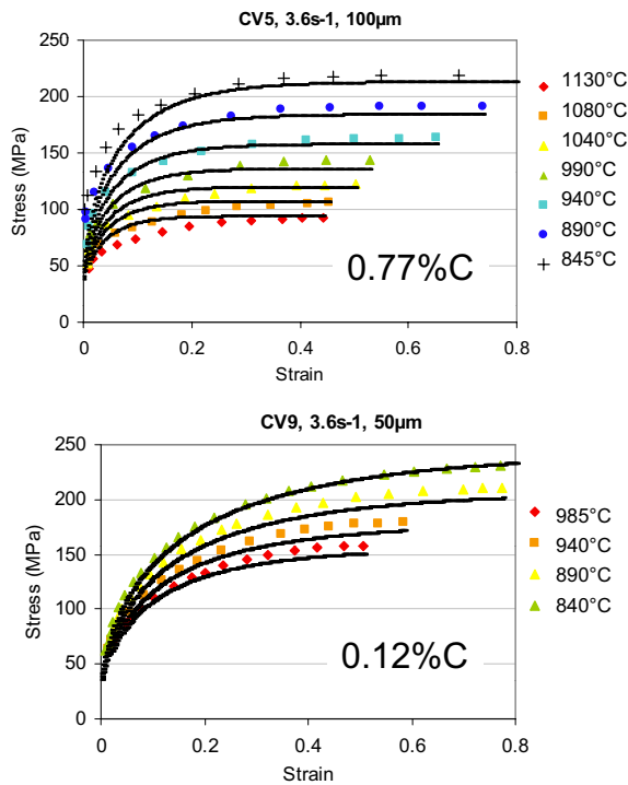
Fig. 2. The carbon level affects the strain hardening of austenite, which is well taken into account by the model (torsion data).
