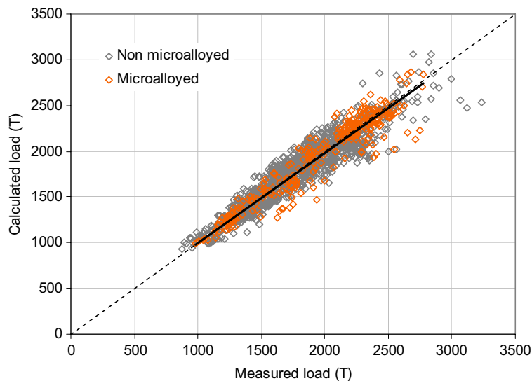
Fig. 4. Good agreement between calculated and measured loads, as measured on the second stand of an industrial finishing mill.
