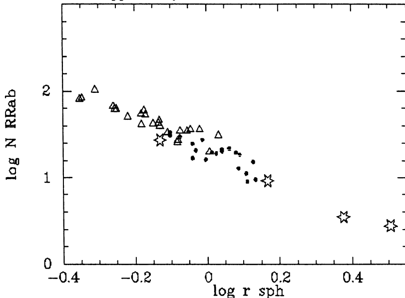
Fig. 1 - Surface density distribution of RR Lyrae type ab in the bulge from Alard (1997) –full circles–, from MACHO –open triangles–, and from Wesselink (1987) –stars–. The RR Lyrae of the Sgr dwarf galaxy are not included in these counts.
