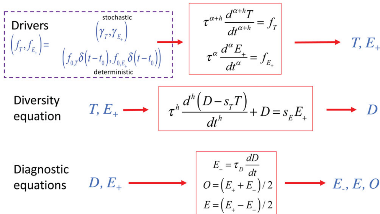
Figure 1. A schematic showing the way the various parts of the Fractional MacroEvolution Model (FMEM) fit together. The basic drivers are shown at the top; physical drivers are the temperature ( T ) and turnover rate ( E_+ ). These are shown at the right, because they have nontrivial properties, such that they are best modeled as the responses to more elementary causes—the temperature and turnover rate forcings ( f_T, f_{E_+} ). In the paper, we primarily discuss the simple case that reproduces the Paleobiology Database (PBDB) statistics, where these are Gaussian white noises ( f_T = \gamma_T, f_{E_+} = \gamma_{E_+} ). However, deterministic forcings such as bolide impacts are also discussed, shown here with both T and E_+ forced with a Dirac function of amplitude f_{0,T}, f_{0,E_+} , respectively. More general forcings can be used and their responses can be obtained using the impulse response functions. The middle line shows how the T, E_+ drivers determine the diversity ( D ). Finally, to complete (close) the model, we need a diagnostic equation that enables us to determine E_-, E, O ; this is shown in the bottom line.
