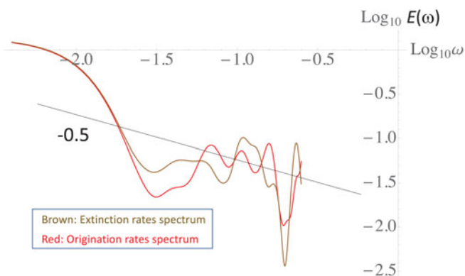
Figure A3.2. Extinction (brown) and origination rates (red) obtained by the Lomb-Scargle method using a Hanning window. The frequencies higher than (4 \text{ Myr})^{-1} were not shown, as they are at higher frequencies than the mean resolution.
