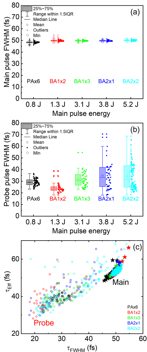
Figure 3. On-shot main and probe pulse measurements during one experimental day in several laser modes. The box-and-whisker plots of the main pulse (a) and probe pulse (b) FWHM durations versus the laser mode and main pulse energy. The colored bars represent the 25%–75% ranges, the error bars are the 1.5 interquartile ranges, the horizontal lines are the medians and the squares, dots and circles are the means, outliers and minima, respectively. The dots on the right from the boxes-and-whiskers are the individual shots forming the corresponding histograms. (c) Main (stars) and probe (rings) pulses on the [FWHM, effective pulse width] plane; each point is an individual shot. Color encodes the laser mode.
