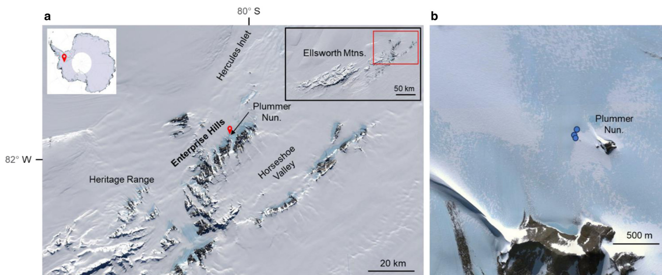
Figure 5. (a) Overview of Enterprise Hills. The red pin in the main image indicates the location of Plummer Nunatak. The red box in the inset map in the upper right highlights the area shown in the main image. (b) Enhanced map showing blue ice area around Plummer Nunatak. Blue dots indicate drill site locations. Base maps for both panels were created from Google Earth: Imagery © 2023 Maxar.
