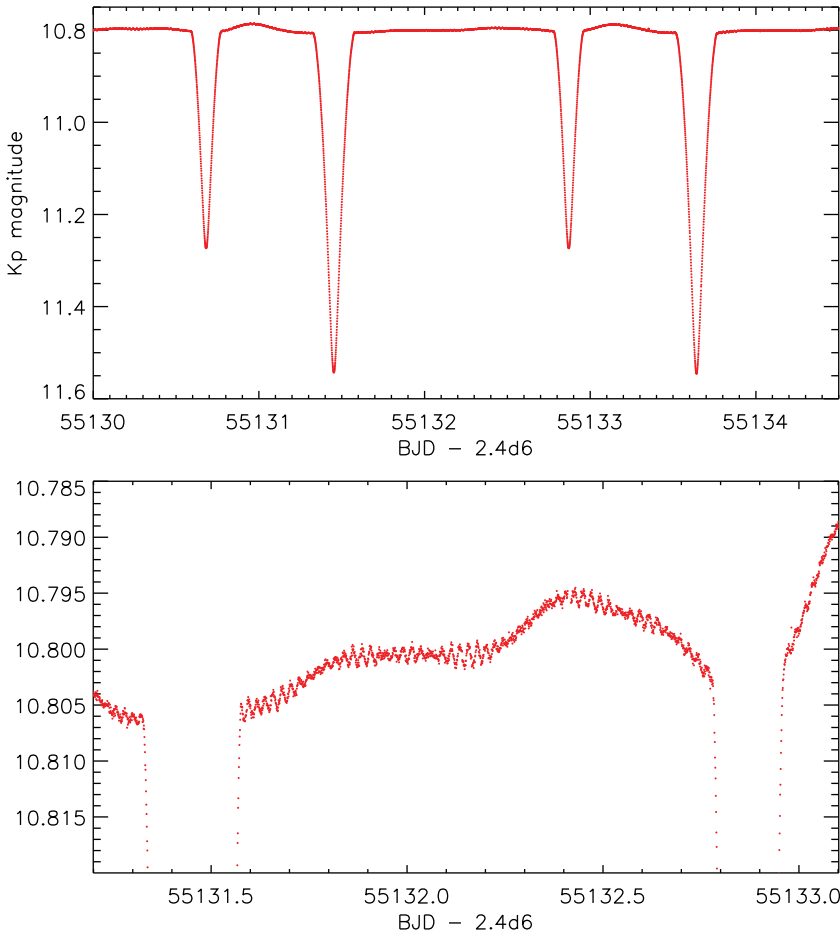
Figure 5. Kepler light curve of KIC 4544587, which shows eclipses, \delta Scuti and \gamma Dor pulsations. Top: part of the short-cadence observations. Bottom: close-up of an short stretch of data outside eclipse.
