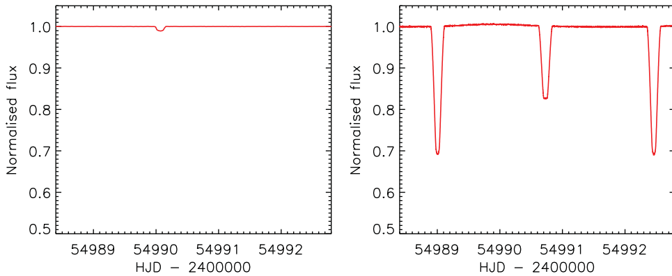
Figure 2. Kepler satellite light curves of the transiting planetary system Kepler-6 (left) and the EB KIC 5288543 (right) on the same axis scales.
