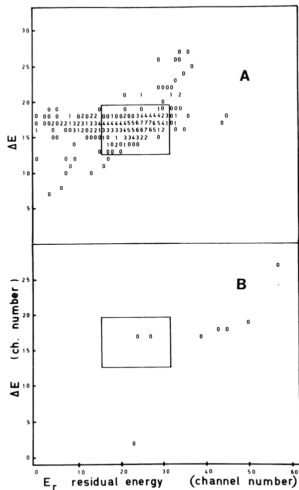
Fig 2. (A) Spectra of \Delta E vs E_r (residual energy) for \text{Al}_2\text{O}_3 standard having ^{26}\text{Al}/^{27}\text{Al} = 4.87 \times 10^{-10} . The numbers in the spectra (n) indicate the number of events in a given channel (N) through the relationship 2^{n-1} < N \leq 2^n . The number of events in ^{26}\text{Al} window is 1009. (B) Spectra of blank \text{Al}_2\text{O}_3 giving ^{26}\text{Al}/^{27}\text{Al} \sim 7 \times 10^{-14}
