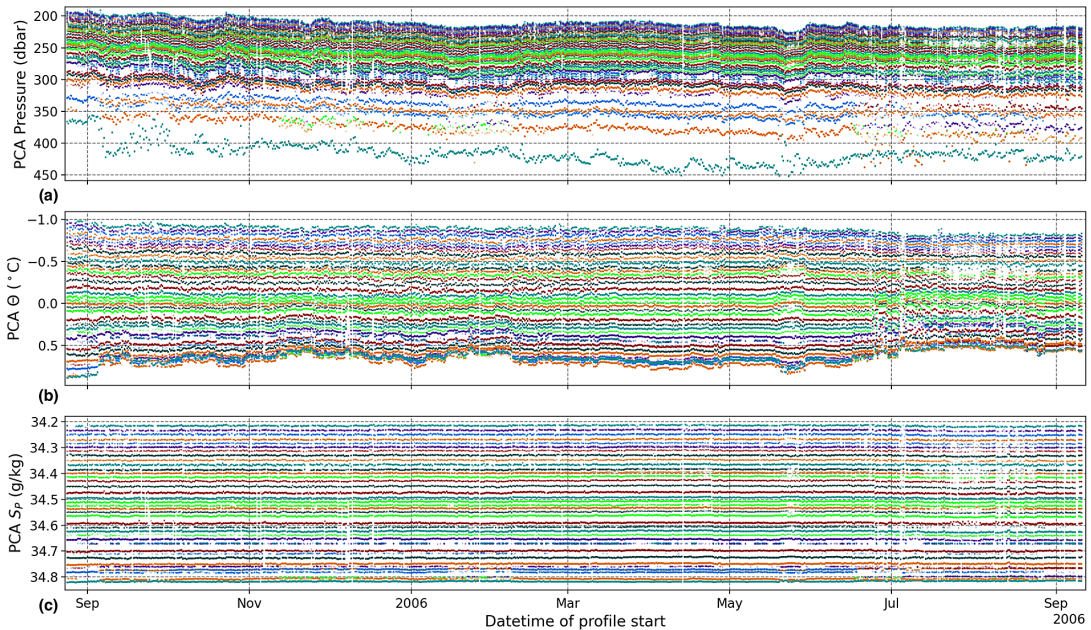
Figure 4. The average (a) pressure, (b) \Theta , and (c) S_p for the points within each cluster for each profile (profile cluster average, PCA) across time. The clustering algorithm was run with m_{pls} = 580 and \ell = 100 dbar on 678,575 data points in the salinity range of 34.21–34.82 g/kg from all up-going ITP3 profiles.
