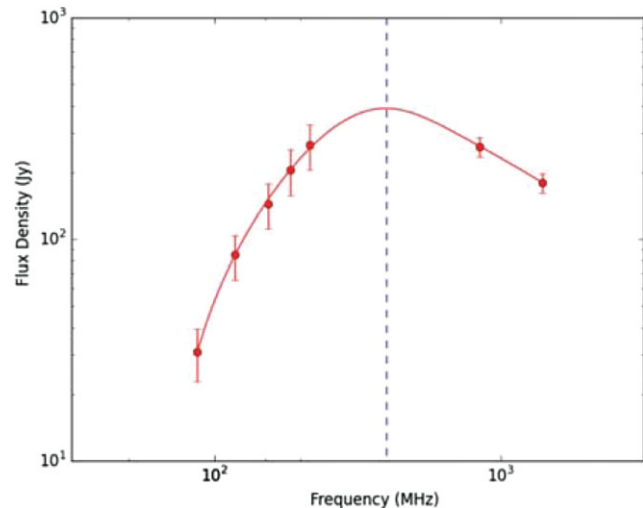
Figure 9. We show the turnover frequency of the H III region G305. The integrated flux density is shown by red symbols. The red line shows the best fit to the data. The vertical blue dashed line shows the turnover frequency of 390 \pm 30 MHz.
