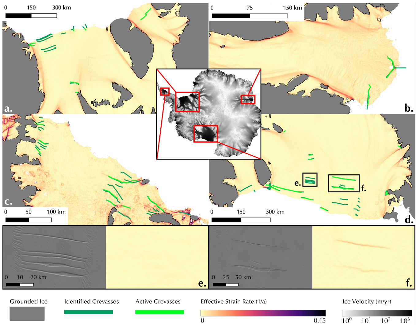
Fig. 1. Fractures observed via optical imagery (dark green) and strain rate (neon green) data over the four ice shelves of interest: (a) Ronne-Filchner (RFIS), (b) Amery (AIS), (c) Larsen C (LCIS), and (d) Ross (RIS). Ice upstream of the grounding line is masked in grey (Morlighem, 2019) and not considered in estimates of ice strength. (e) An example of identified crevasses on the RIS as seen on MOA2014 (left) and strain rate fields (right). (f) An example of active crevasses on the RIS as seen on MOA2014 (left) and strain rate fields (right). The inset in (a)-(d) shows ice velocity over Antarctica (Rignot and others, 2017), with the aforementioned ice shelves boxed in red. We do not mask grounded ice in the inset.
