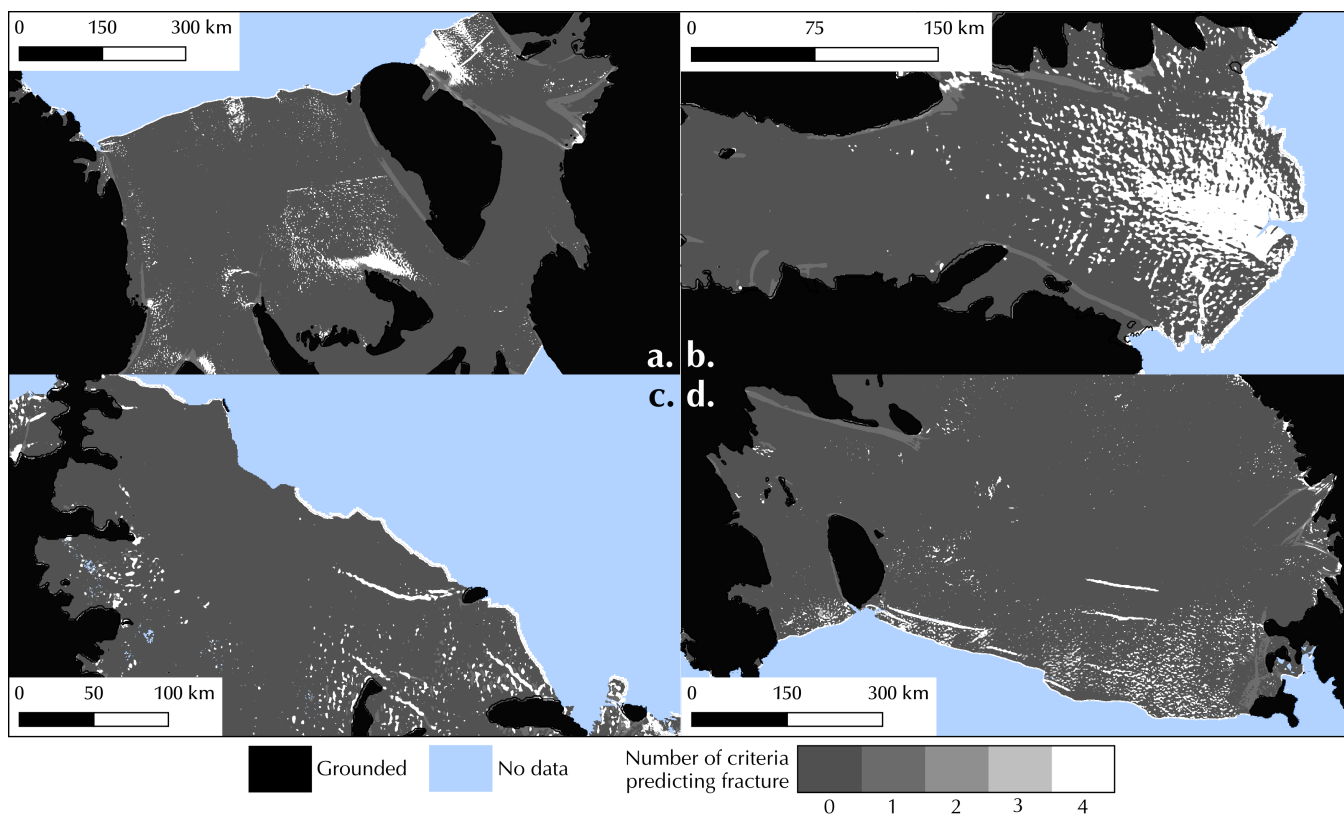
Fig. 5. A map of predicted fracture areas for n=4 on the (a) Ronne-Filchner, (b) Amery, (c), Larsen C, and (d) Ross Ice Shelves. White represents areas where all four yield criteria predict the ice will fracture, and dark grey represents areas where no criteria predict fracture will occur.
