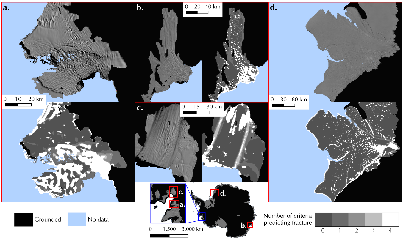
Fig. 6. MODIS 2014 imagery (top [a,d]; left [b,c]) and our predicted fracture map (bottom [a,d]; right [b,c]) of four smaller ice shelves originally outside of the study area: (a) Thwaites (b) Totten (c) Pine Island, and (d) Brunt
