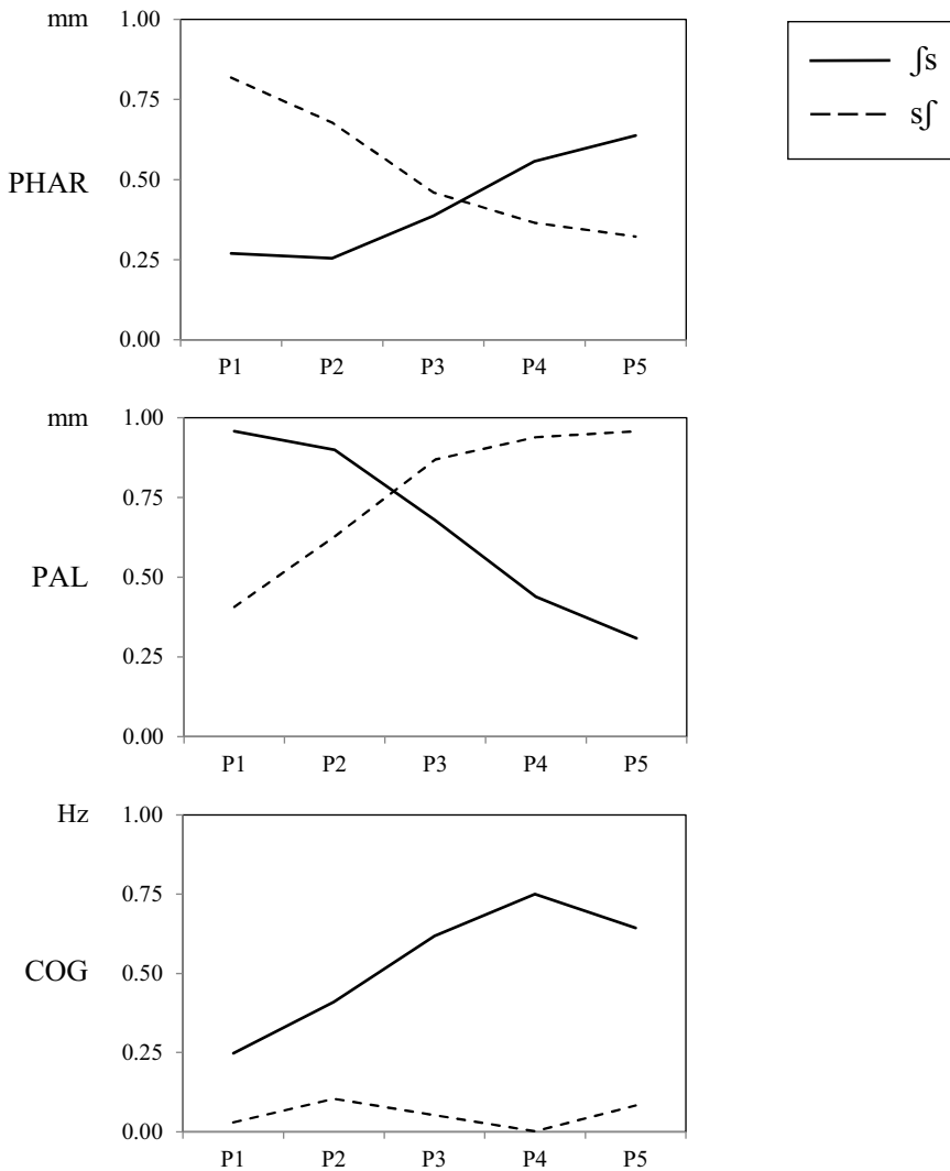
Figure 5. Normalized tongue position and COG values for /ʃ#s/ and /s#ʃ/ at the temporal points P1, P2, P3, P4 and P5 across subjects. Values for /ʃ#s/ are set to 1 and those for /s#ʃ/ to 0 for the PHAR and COG signals, and the reverse for PAL.
