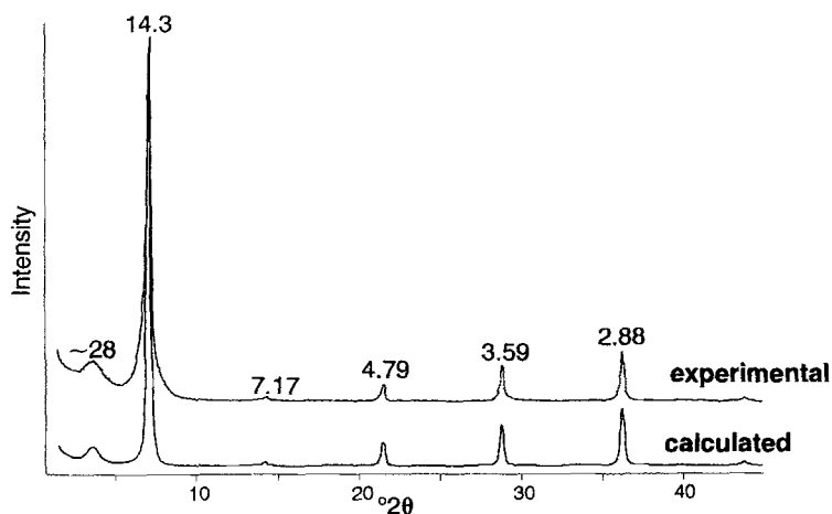
Figure 5. Calculated X-ray traces of vermiculite and unusual 28 \text{ \AA} domain. The calculated pattern represents a mixture of regular vermiculite (93 vol.%) and 28 \text{ \AA} edge layers (7 vol.%). \text{CoK}\alpha radiation.
