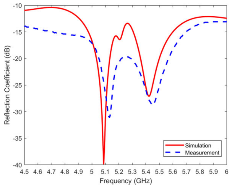
Fig. 14. Simulated and measured reflection coefficients of the circularly polarized eighth-mode substrate integrated waveguide antenna.
