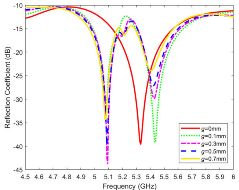
Fig. 10. Simulated reflection coefficients for different values of gap spacing g of the circularly polarized eighth-mode substrate integrated waveguide antenna.
