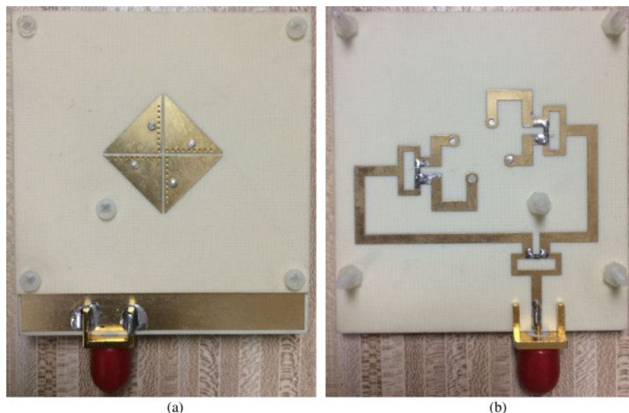
Fig. 13. Photographs of the fabricated CP EMSIW antenna. (a) Radiator on the top layer. (b) Power divider on the bottom layer.
