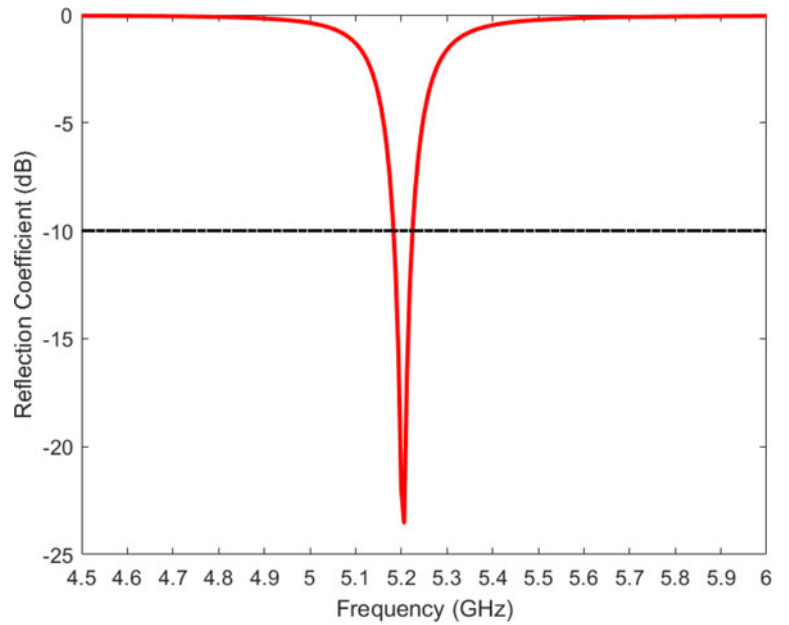
Fig. 6. Simulated reflection coefficient of the linearly polarized eighth-mode substrate integrated waveguide antenna.
