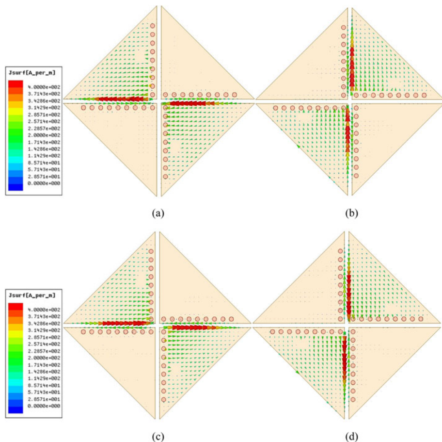
Fig. 12. Simulated electric current distribution on the patch of the circularly polarized eighth-mode substrate integrated waveguide antenna at different phases of 5.2 GHz. (a) Phase = 30°. (b) Phase = 120°. (c) Phase = 210°. (d) Phase = 300°.
