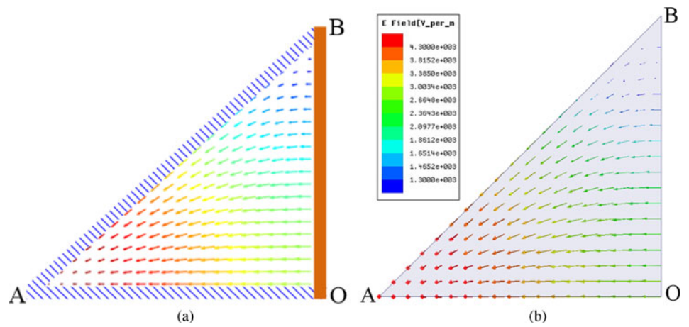
Fig. 2. Electric field lines for the TM_{11} mode in the isosceles right triangular waveguide with two magnetic walls and one electric wall on a cathetus. (a) Analytically calculated electric field lines. (b) Simulated electric field lines.
