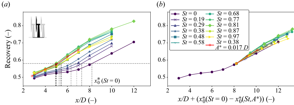
Figure 9. Evolution of wake recovery against downstream position for surge motion with different St (a) and virtual origin-based rescaling (b). Panel (a) shows the recovery evolution together with the position of x_0^* marked by the dotted lines (downstream position where the recovery is R_0^* = 0.58 ). Panel (b) displays the same plot as for (a) but with a shift of the recovery curves based on x_0^* . Cases D.1, D.2 and D.2* with St \in [0, 0.97] , A^* = 0.007 and St = 0.38 , A^* = 0.017 from table 3 are displayed, with Re = 1.4 \times 10^5 .
