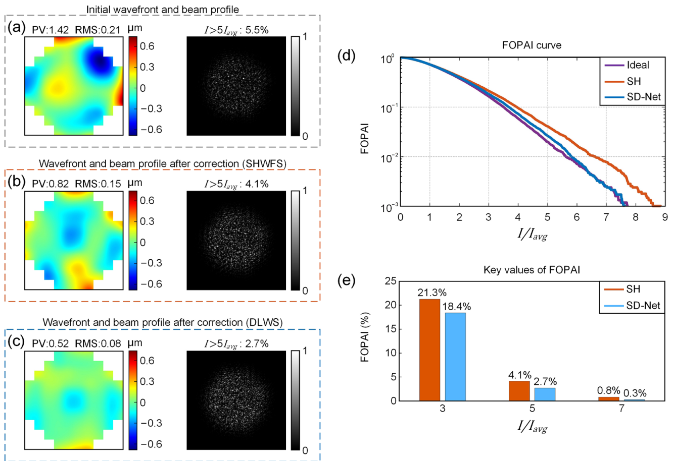
Figure 8. Wavefront correction results using the DLWS method and SHWFS. (a) Initial wavefront distortion and beam profile. (b) Wavefront reconstruction error and beam profile of the SHWFS. (c) Wavefront reconstruction error and beam profile of the DLWS method. (d) FOPAI curves. (e) Key parameters of FOPAI.
