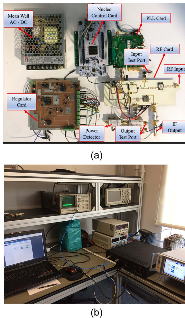
Figure 9. (a) The circuit design of the proposed frequency down-converter and (b) the measurement setup of proposed X-band frequency down-converter.
