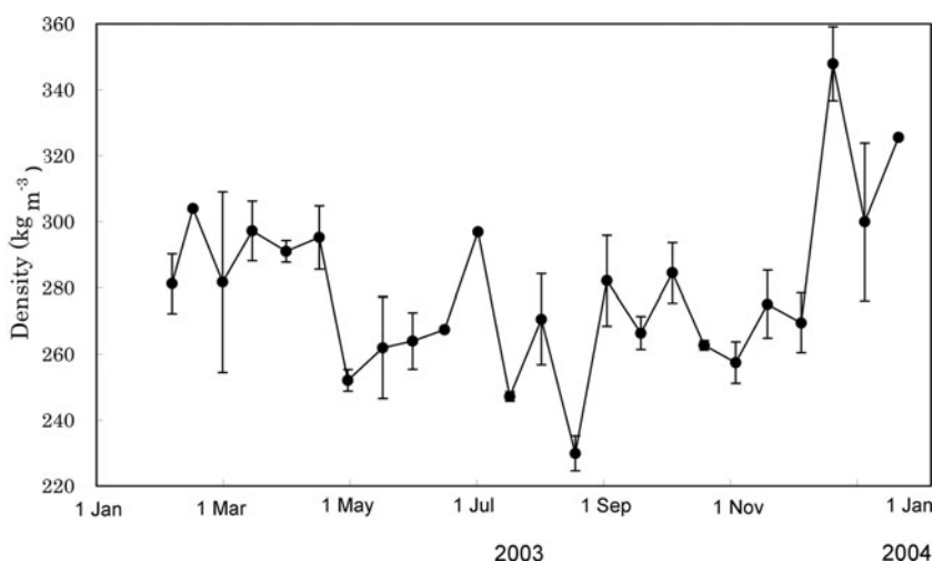
Fig. 3. Snow density from the surface to 10 cm depth at Dome Fuji in 2003. The average value was 280 kg m -3 .
