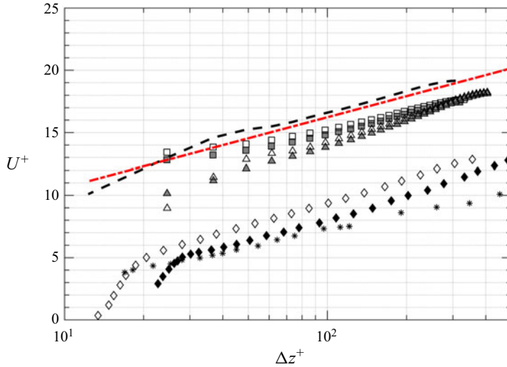
Figure 6. Inner-scaled mean streamwise velocity. Symbols as in figure 5; *, boundary layer with p/k = 3.33 (Keirbulck et al. 2002), \blacklozenge and \diamond , channel flow with p/k = 8 at Re_\tau = 400 and 600 , respectively (Krogstad et al. 2005).
