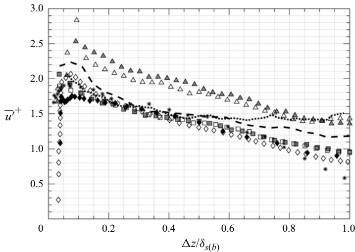
Figure 7. Streamwise velocity fluctuations \overline{u'}^+ = \sqrt{u'^2}/u_s^* modified by different coverages. Symbols as in figure 5 and 6.
