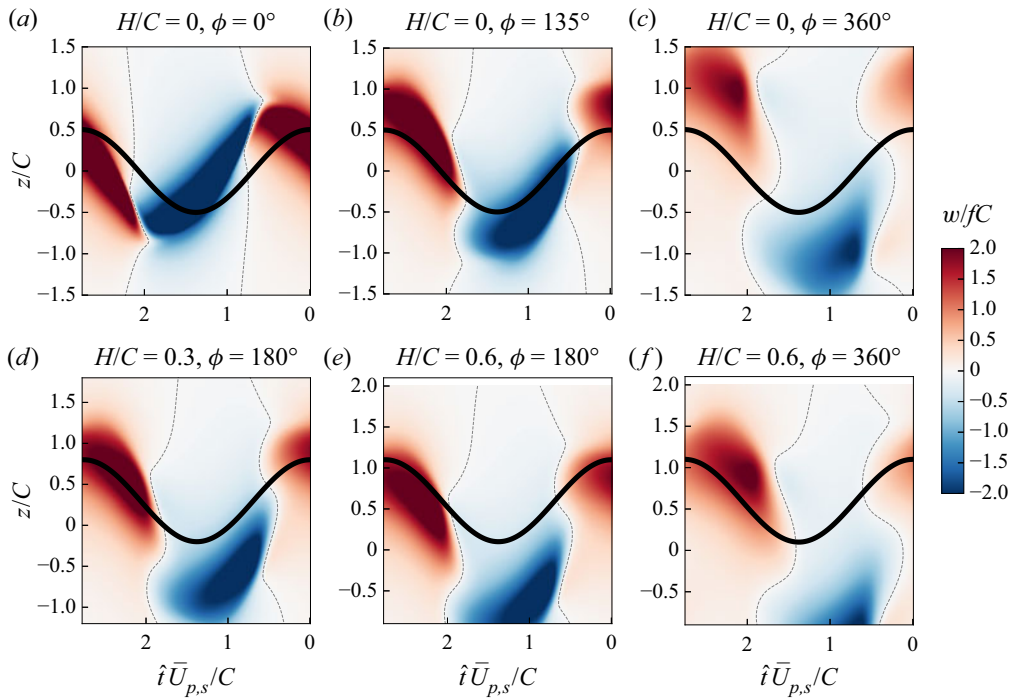
Figure 8. Vertical velocity field at y = 0 seen by the leading edge of the follower’s flapper as if it were in the undisturbed wake of the isolated flapper. Black line denotes the vertical position of the follower’s leading edge as a function of time, where \hat{t} = 0 is the beginning of the follower’s downstroke. Dashed black lines are the contours for w = 0 .
