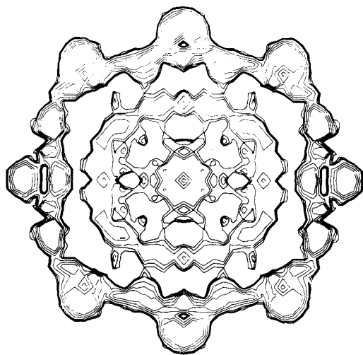
The distribution of protein in tomato bushy stunt virus (TBSV) at 16 Å resolution. Section through the centre of the virus particle in 70% D 2 O/H 2 O where the RNA is contrast matched
