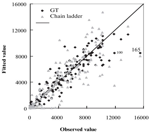
FIGURE 6: Observed y_{ij} versus predicted E(y_{ij}) losses for the GT and chain ladder models.
