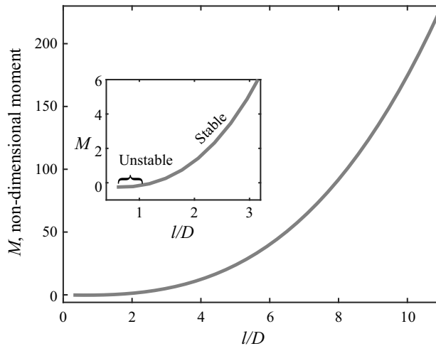
Figure 12. Net moment M > 0 shows that the cylinder is in stable equilibrium. Net moment M acting on horizontal cylinder with \theta = 150^\circ , D = 1.5 mm and \rho_s = 4000 kg m -3 floating at an air–water interface at various aspect ratios. The inset shows the enlarged view of moment M at small aspect ratios.
