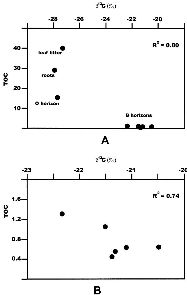
Figure 11 A: Scatter plot of \delta^{13}\text{C} vs. % TOC values from all horizons, roots, and leaf litter; R^2 = 0.80 ; B: Scatter plot of \delta^{13}\text{C} vs. % TOC values from B horizons only; R^2 = 0.74
