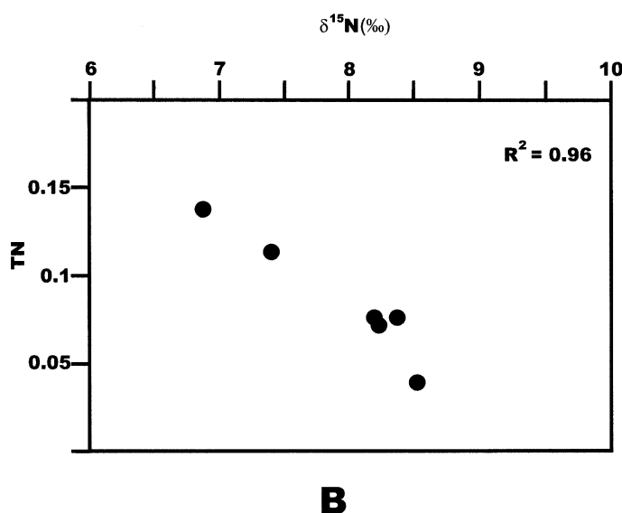
Figure 9 A: Scatter plot of \delta^{15}\text{N} vs. % TN values from all horizons, roots, and leaf litter; R^2 = 0.80 ; B: Scatter plot of \delta^{15}\text{N} vs. % TN values from B horizons only; R^2 = 0.96
