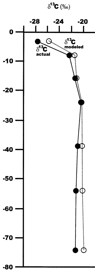
Figure 12 Depth profiles of predicted \delta^{13}\text{C} values and actual \delta^{13}\text{C} values; R^2 = 0.95
