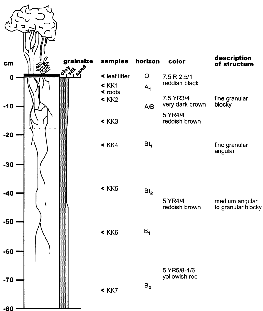
Figure 3 Kakamega Forest soil profile, showing sample numbers and depths, grainsize estimates, soil horizons, soil color, and description of soil textures
