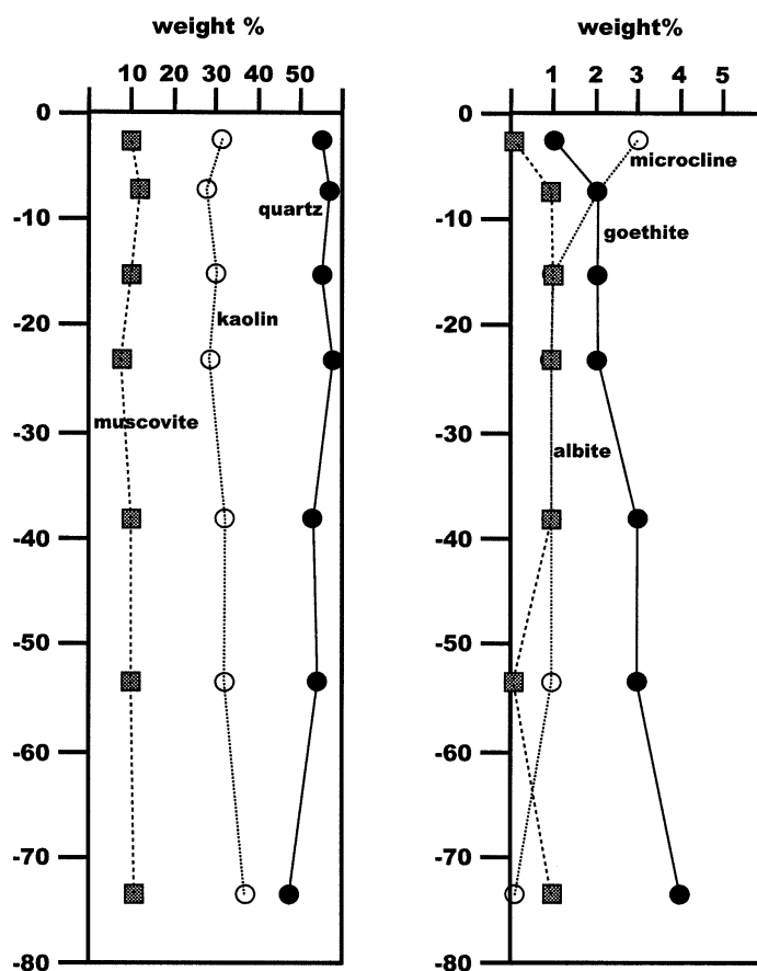
Figure 4 XRD depth profiles for quartz, kaolin, muscovite, microcline, goethite, and albite
