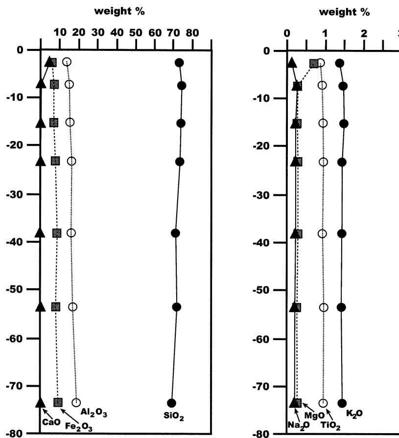
Figure 5 XRF depth profiles for \text{SiO}_2 , \text{Al}_2\text{O}_3 , \text{Fe}_2\text{O}_3 , \text{CaO} , \text{K}_2\text{O} , \text{MgO} , \text{TiO}_2 , and \text{Na}_2\text{O}
