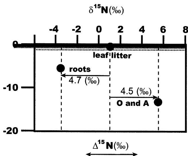
Figure 10 \Delta^{15}\text{N} differences between leaf litter, roots, and O and A horizons
