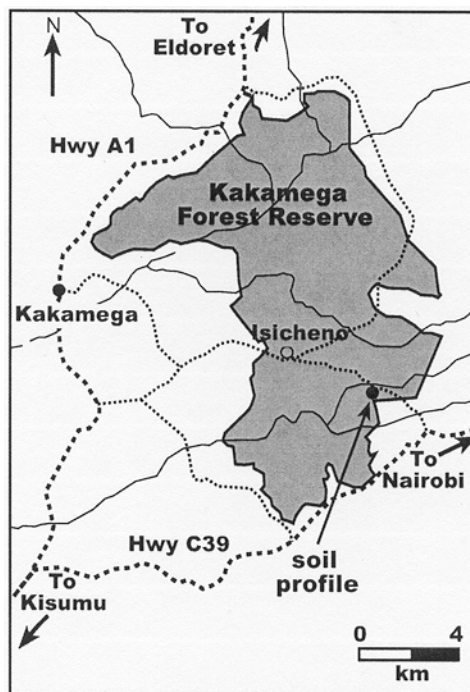
Figure 2 Location of sampling site within the Kakamega Forest Reserve
