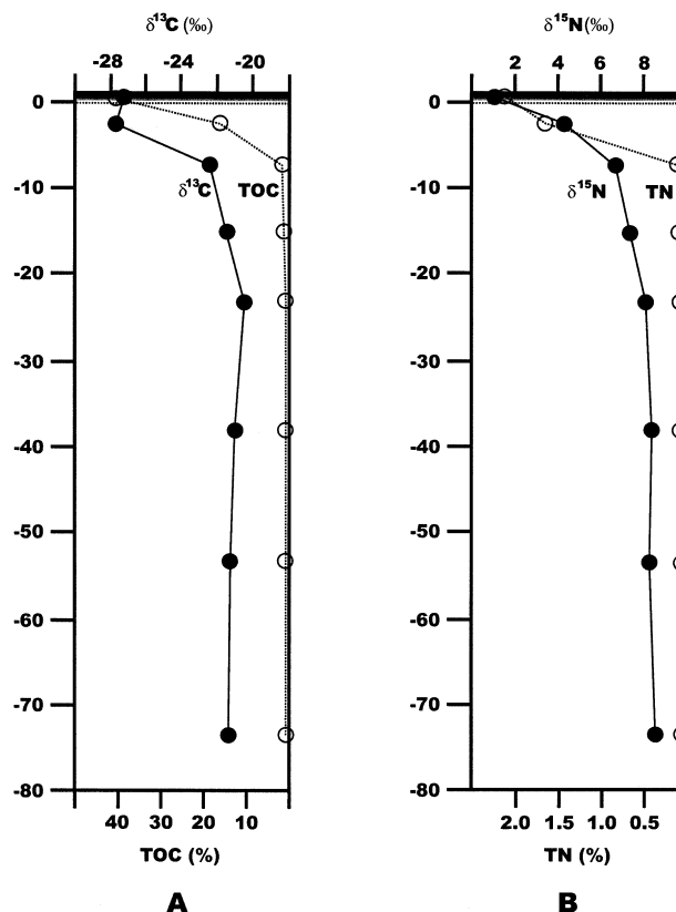
Figure 8 A: Depth profiles of acid treated \delta^{13}\text{C} and TOC values; B: Depth profiles of non-acid treated \delta^{15}\text{N} and TN values
