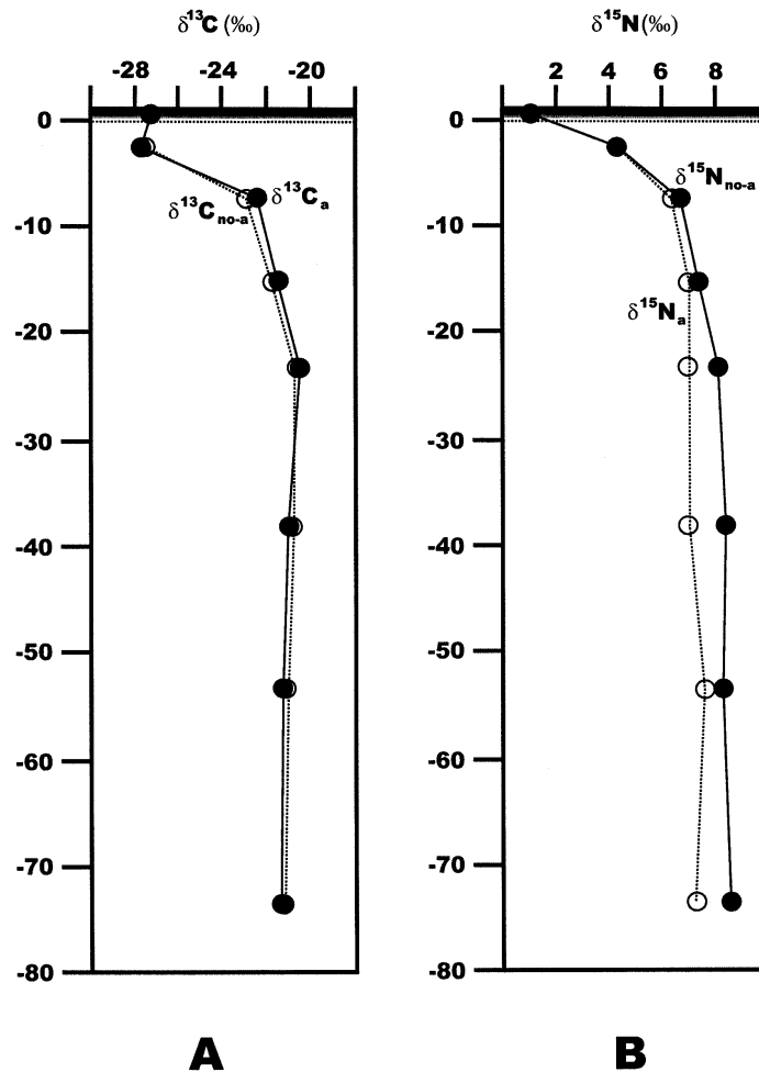
Figure 6 A: Depth profiles of acid-treated and non-acid treated \delta^{13}\text{C} values; B: Depth profiles of acid-treated and non-acid treated \delta^{15}\text{N} values
