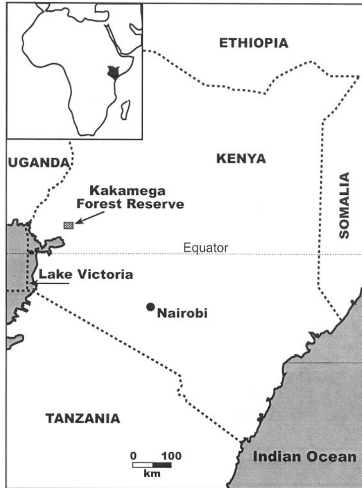
Figure 1 Location of Kakamega Forest in the western part of Kenya
