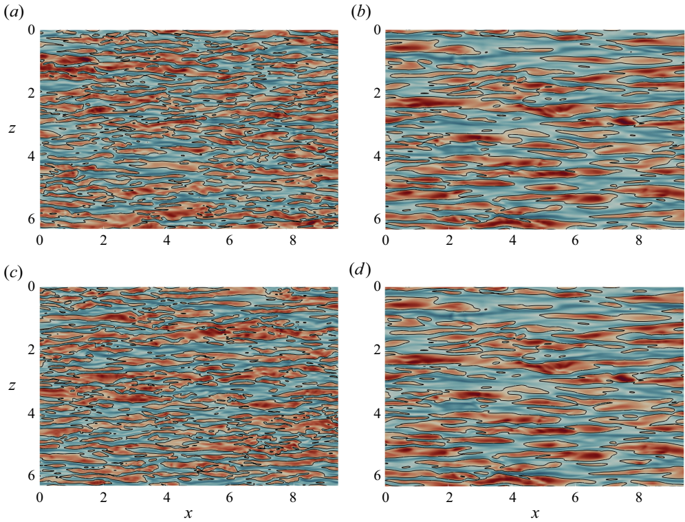
Figure 3. Streamwise velocity fluctuations u^+ in a wall-parallel portion of the x - z plane at y^+ = 10 for ZBC (a,b) and CBC (c,d) at M_w^b = 0.3 (a,c) and M_w^b = 1.5 (b,d) for the uncontrolled case. The blue-to-red colour scale ranges from -10 to +10 ; the black line is for the zero contour level.
