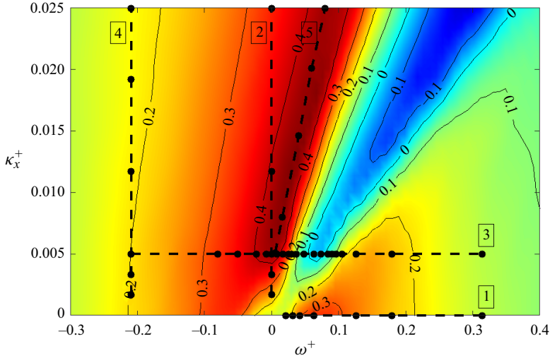
Figure 1. Incompressible drag reduction vs \kappa_x^+ and \omega^+ , at A^+ = 12 and Re_\tau = 400 . The map is obtained from Gatti & Quadrio (2016) via interpolation of their datasets at Re_\tau = 200 and Re_\tau = 1000 . The dots on the dashed lines correspond to the present compressible simulations.
