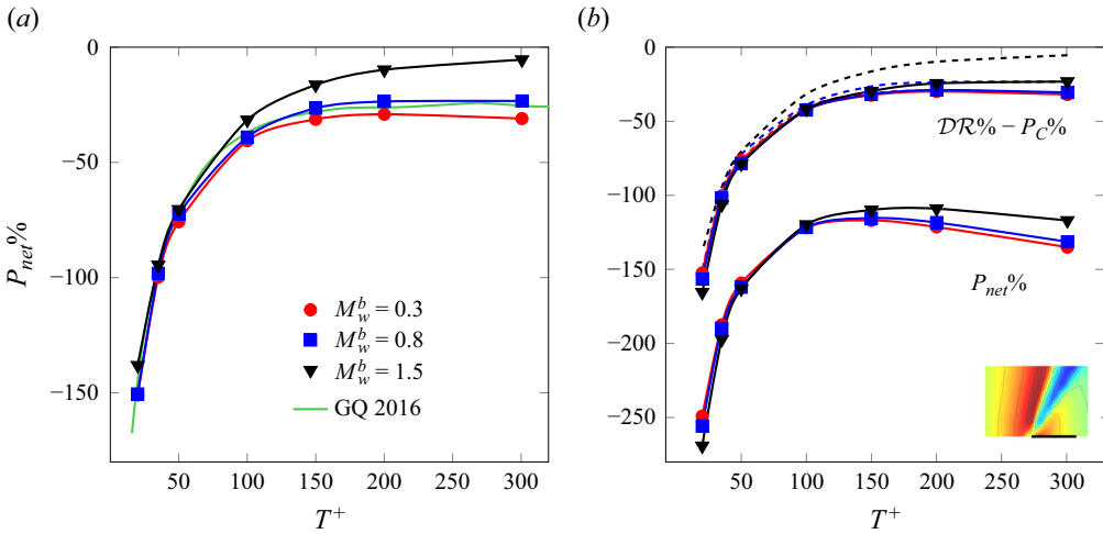
Figure 12. Net power saving for the oscillating wall (line 1 of figure 1, see inset), for ZBC (a) and CBC (b). Incompressible data are in green; (b) also plots DR\% - P_c\% (top set of curves), where dashed lines are for ZBC.
