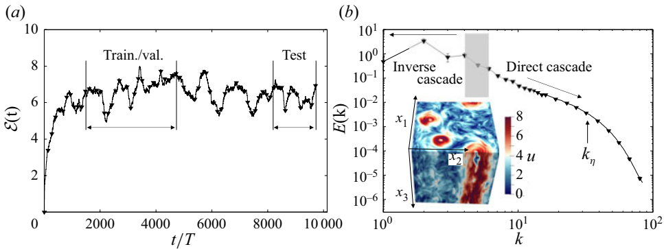
Figure 2. (a) Energy evolution of the turbulent flow, where we also show the sampling time periods for the training/validation and testing data. (b) The averaged energy spectrum. The grey area indicates the forcing wavenumbers, and k_\eta is the Kolmogorov dissipative wavenumber where E(k) starts to decay exponentially. The inset shows an instantaneous visualization of the velocity module with the frame of reference for the simulation.
