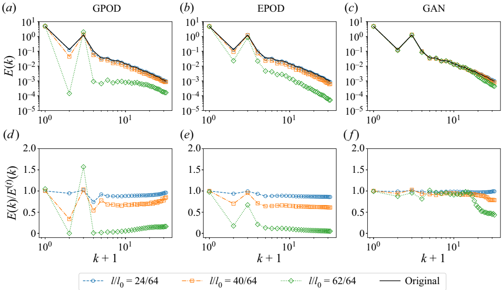
Figure 15. Energy spectra of the original velocity module and the reconstructions obtained from GPOD, EPOD and GAN for a square gap of different sizes (a–c). The corresponding E(k)/E^{(t)}(k) is shown in (d–f), where E(k) and E^{(t)}(k) are the spectra of the reconstructions and the ground truth, respectively.
