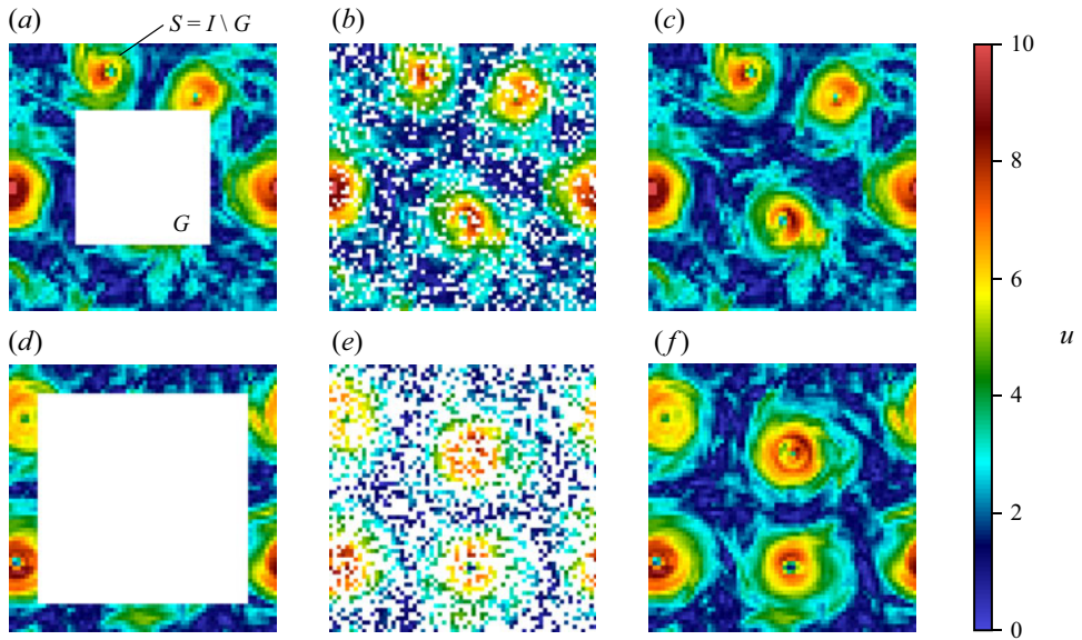
Figure 1. Examples of the reconstruction task on 2-D slices of 3-D turbulent rotating flows, where the colour code is proportional to the velocity module. Two gap geometries are considered: (a,d) a central square gap and (b,e) random gappiness. Gaps in each row have the same area and the corresponding ground truth is shown in (c,f). We denote G as the gap region and S = I \setminus G as the known region, where I is the entire 2-D image.
