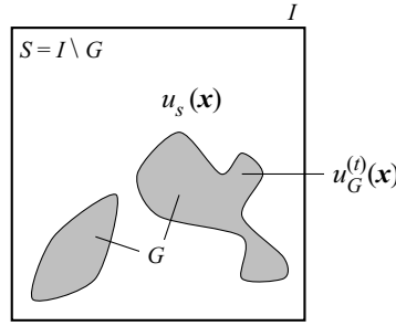
Figure 3. Schematic diagram of a gappy field.
