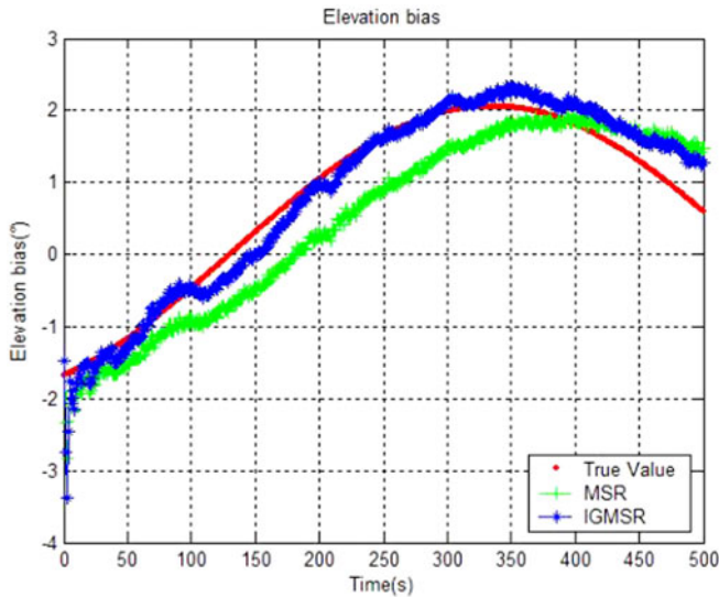
Figure 4. Elevation bias estimation results of the two algorithms.
