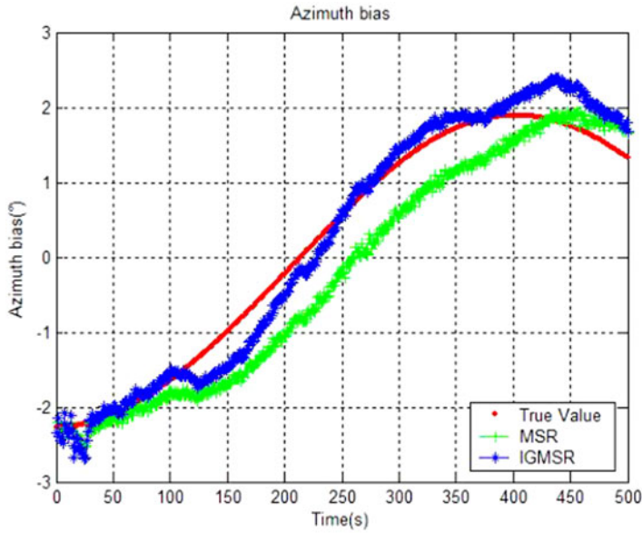
Figure 3. Azimuth bias estimation results of the two algorithms.
