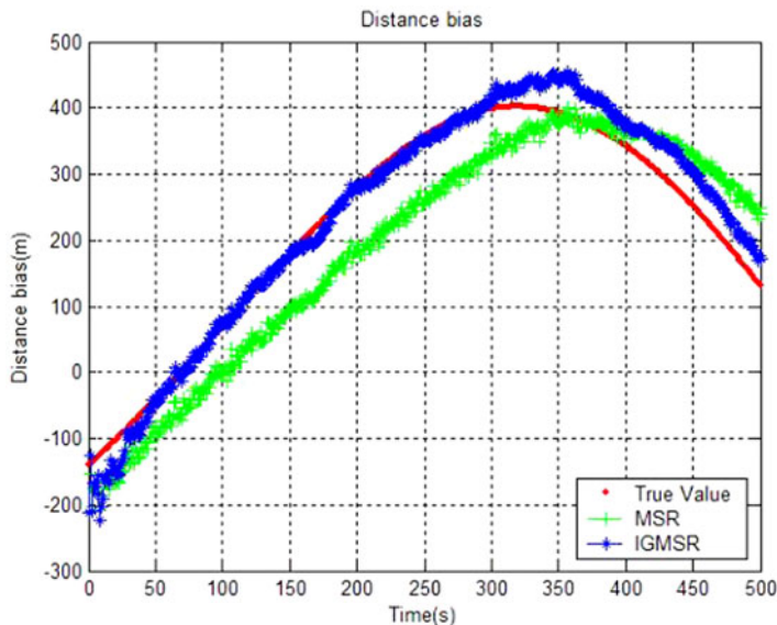
Figure 2. Distance bias estimation results of the two algorithms (Algorithm 1 refers to the MSR).
