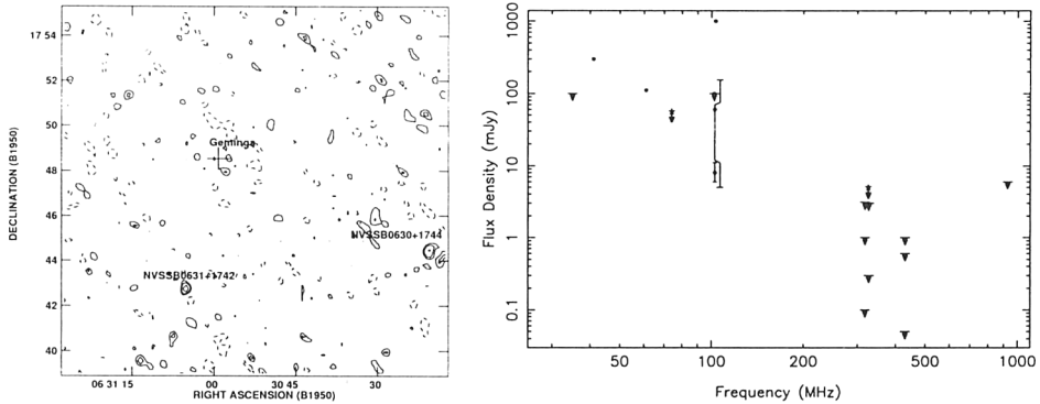
Figure 1. ( Left ) Geminga at 74 MHz. The angular resolution is 25'' , and the rms noise level is 28 \text{ mJy beam}^{-1} . The cross marks the location of the optical counterpart (Caraveo et al. 1998), and the sources NVSS B0630+1744 and B0631+1742 are marked for reference. The 326 MHz image is similar. ( Right ) The spectrum of Geminga.
