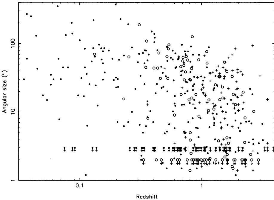
Figure 1. The angular size – redshift plot for radio galaxies (‘•’ measured z , ‘+’ estimated z ) and quasars (o) with known z in the MRC 1-Jy samples.
