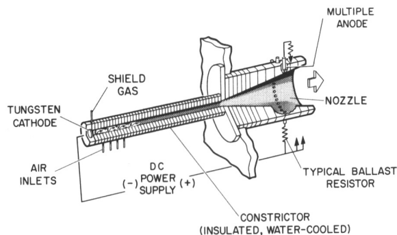
FIGURE 1.—Schematic drawing of a constricted-arc supersonic jet.
