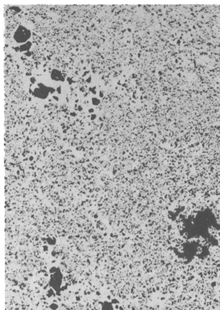
FIGURE 7.—Polished sections of "magnetite" and "hematite" models.
