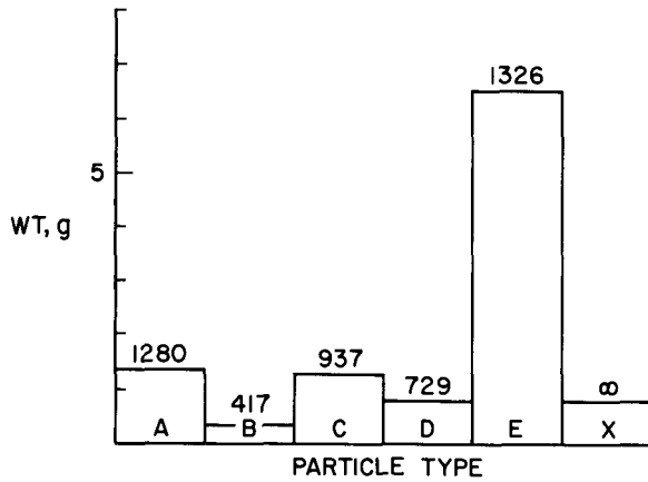
FIGURE 4.—Collected debris from magnetite model.
