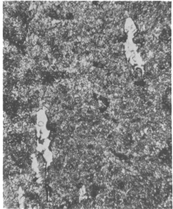
FIGURE 6.—Flattened droplet with micron size splatter drops.
