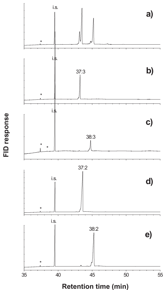
Figure 7 Partial GC/FID traces of alkenones isolated by HPLC from Black Sea sediments: a) initial mixture of alkenones; b) fraction 2 (13–14 min); c) fraction 4 (15–16 min); d) fraction 6 (17–18 min); e) fraction 8 (19–20 min).
