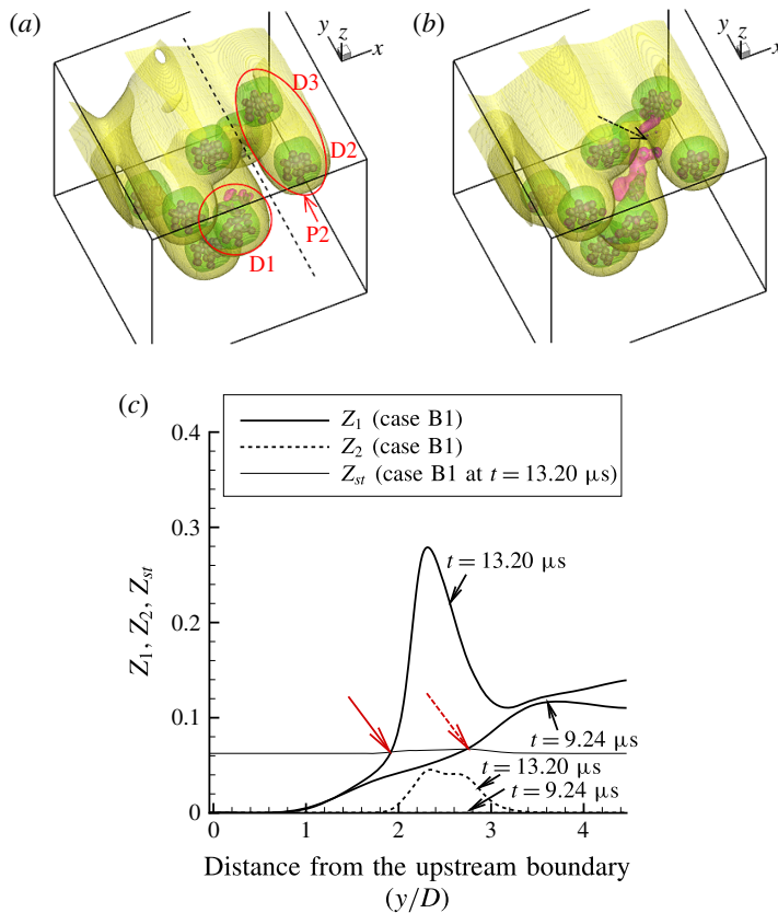
FIGURE 18. (Colour online) Puffing effects on droplet grouping in case B1. In (a) and (b), the yellow isosurface represents the stoichiometric surface and the pink isosurface represents Y_{\text{ethanol}} = 0.05 : (a) t = 9.24 \mu\text{s} ; (b) t = 13.20 \mu\text{s} . The dashed line in (a) indicates the region where data samples are obtained to plot the mixture fraction profiles Z_1 , Z_2 and Z_{st} in (c).
