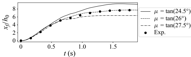
Figure 30. Granular collapse on slope angle \theta = 22^\circ using rate-independent MCC with constant slope \mu of CSL, otherwise using the parameters as in § 4.2 treating the rate-dependent case. Experimental data of Mangeney et al. (2010).
