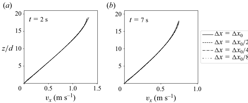
Figure 29. Cohesionless flow on inclination \theta = 28^\circ under grid refinement, using parameters as in table 7. The velocity profile was initially imposed as linear (with a surface velocity of 4 \text{ m s}^{-1} ) and is here shown at two different later times, the right plot being the steady-state profile.
