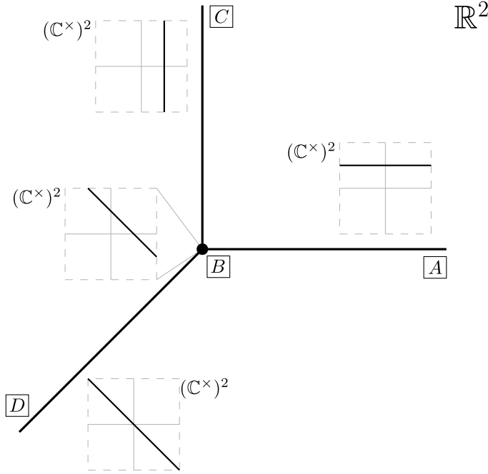
Figure 1. The fine tropical line \text{ftrop}(V^\times(P)) from example 5.5. We view the ambient space (\mathbb{C} \times \mathbb{R})^2 as \mathbb{R}^2 with a copy of (\mathbb{C}^\times)^2 at each point. As such, \text{ftrop}(V^\times(P)) can be viewed as the usual tropical line in \mathbb{R}^2 with the subvariety of the complex torus V^\times(\text{in}_u(P)) attached at each point u \in \mathbb{R}^2 . The labels allow identification with the components given in (5.2) and (5.3).
