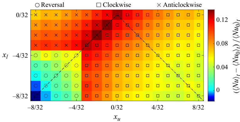
Figure 2. Phase diagram in x_u-x_l plane with values of the effective Nusselt number, defined as Nu_{eff} = (\langle Nu \rangle_t - \langle Nu_0 \rangle_t) / \langle Nu_0 \rangle_t , at Ra = 1 \times 10^8 and Pr = 2 . Crosses and squares correspond to stable anticlockwise and clockwise LSCs, respectively, and circles to detected reversals, where Nu_0 denotes the Nusselt number of the traditional RBC cell at the same Ra and Pr . Here, the initial velocity and temperature fields are \mathbf{u} = 0 and \theta = (\theta_l + \theta_u)/2 , respectively.
