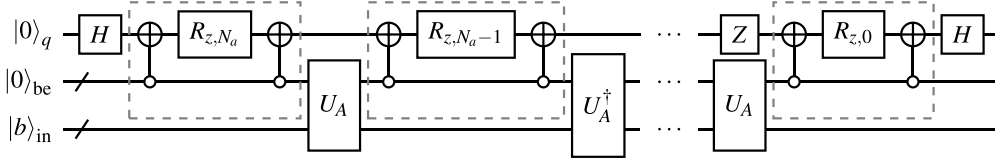
FIGURE 7. The QSVT circuit encoding a real polynomial of order N_a , where N_a is odd, by using N_a + 1 angles \phi_k pre-computed classically. The gates denoted as R_{z,k} represent the rotations R_z(2\phi_k) . For an even N_a , the gate Z should be removed and the rightmost BE oracle U_A should be replaced with its Hermitian adjoint version U_A^\dagger .
