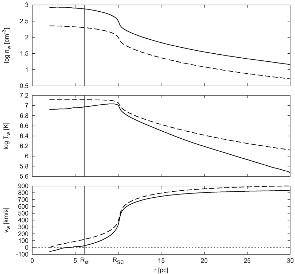
Figure 1. Radial profiles of particle density, temperature and velocity for single-modal (dashed lines) and bi-modal (solid lines) solutions.
