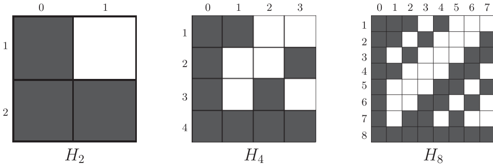
Figure 1. Hadamard matrices of order 2, 4, 8, which are unique up to equivalence. Here, black represents 1 and white represents -1 .
