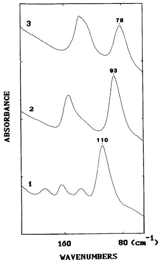
Figure 1. Infrared absorption spectra of (1) muscovite, (2) phlogopite, and (3) biotite in polyethylene pellets between 220 and 20 \text{cm}^{-1} .
