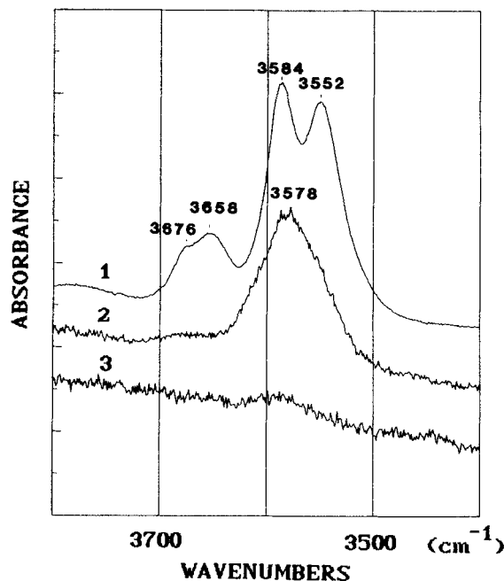
Figure 4. Infrared spectra of (top) K and (bottom) structural-OH groups of biotite as a function of temperature: 1, 30°C; 2, 550°C; 3, 650°C. Upper spectra were obtained in polyethylene pellets; lower spectra, with single crystals.
