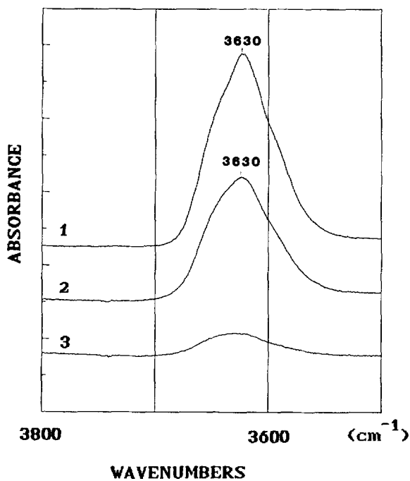
Figure 2. Infrared spectra of (top) K and (bottom) structural-OH groups of muscovite as a function of temperature: 1, 30°C; 2, 650°C; and 3, 750°C. Upper spectra were obtained in polyethylene pellets; lower spectra, with single crystals.
