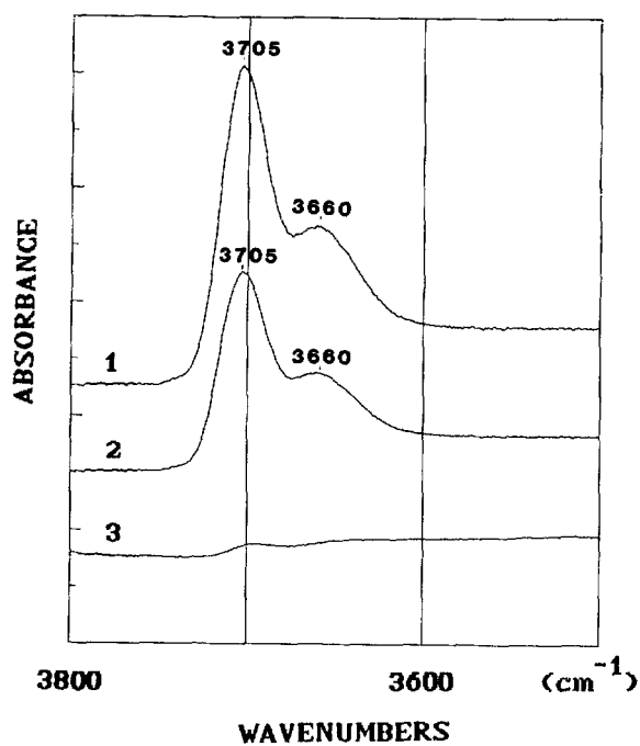
Figure 3. Infrared spectra of (top) K and (bottom) structural-OH groups of phlogopite as a function of temperature: 1, 30°C; 2, 1100°C; 3, 1150°C. Upper spectra were obtained in polyethylene pellets; lower spectra, with single crystals.
