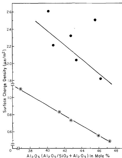
Fig. 2. Variation of surface charge density of imogolite with mole % \text{Al}_2\text{O}_3 .
