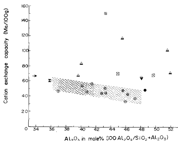
Fig. 1. Variation of cation exchange capacity with mole % \text{Al}_2\text{O}_3 .
