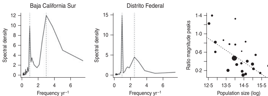
Fig. 5. Spectral density of log reported rubella incidence + 1 for two districts in Mexico, with the resonant and non-resonant peaks shown as vertical dashed lines; and the ratio of the non-resonant peak over the resonant peak across population size for districts where the non-resonant peak was identifiable (26/32 districts). Point size scales inversely with the precision of the second peak (large points correspond to sharp peaks, small points correspond to broad peaks). The equation of the line is y = 3.49 - 0.21x , P < 0.01 , r^2 = 0.26 , and corresponds to a regression weighted by the precision of the second peak (the unweighted regression is also significant).
