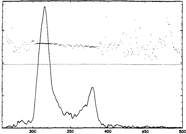
FIGURE 1 The vector averaged, cross-correlation spectrum of H_{30\alpha} maser emission from MWC 349 at 1.29 mm taken with the CSO-JCMT interferometer. The dots mark the phase of each channel on a scale of -\pi to \pi which covers the upper half of the plot. The solid line connects the amplitude points. The full amplitude scale is \sim 125 Jy. Each channel is 0.625 MHz ( 0.81 \text{ km s}^{-1} ) wide.
